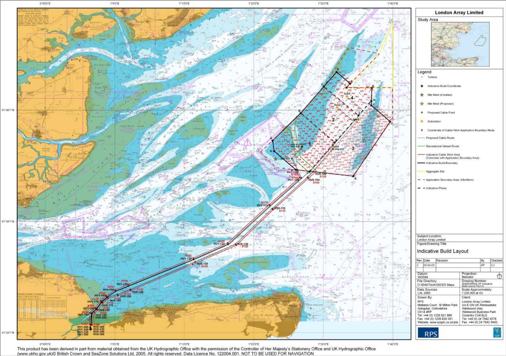
Figure 1. Indicative Build Layout for London Array.
